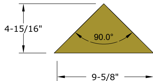
Roof truss gusset
