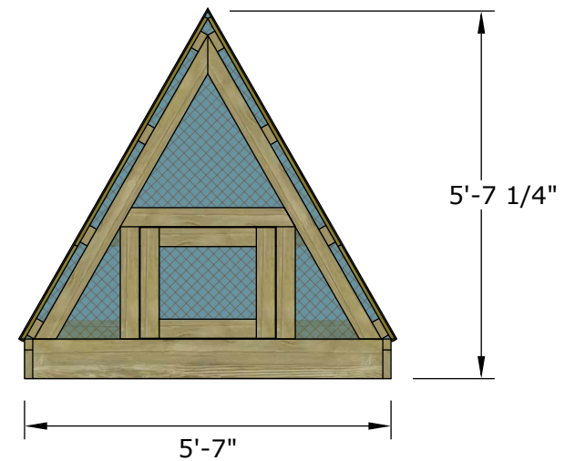
Front Elevation
