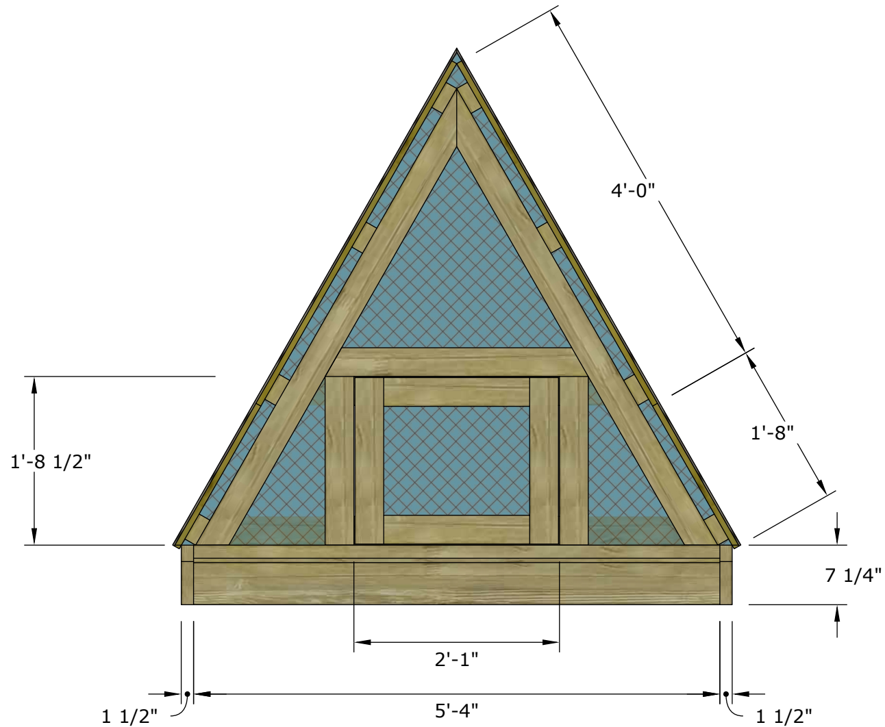
Back Elevation
