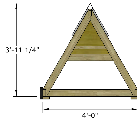
Front Elevation
